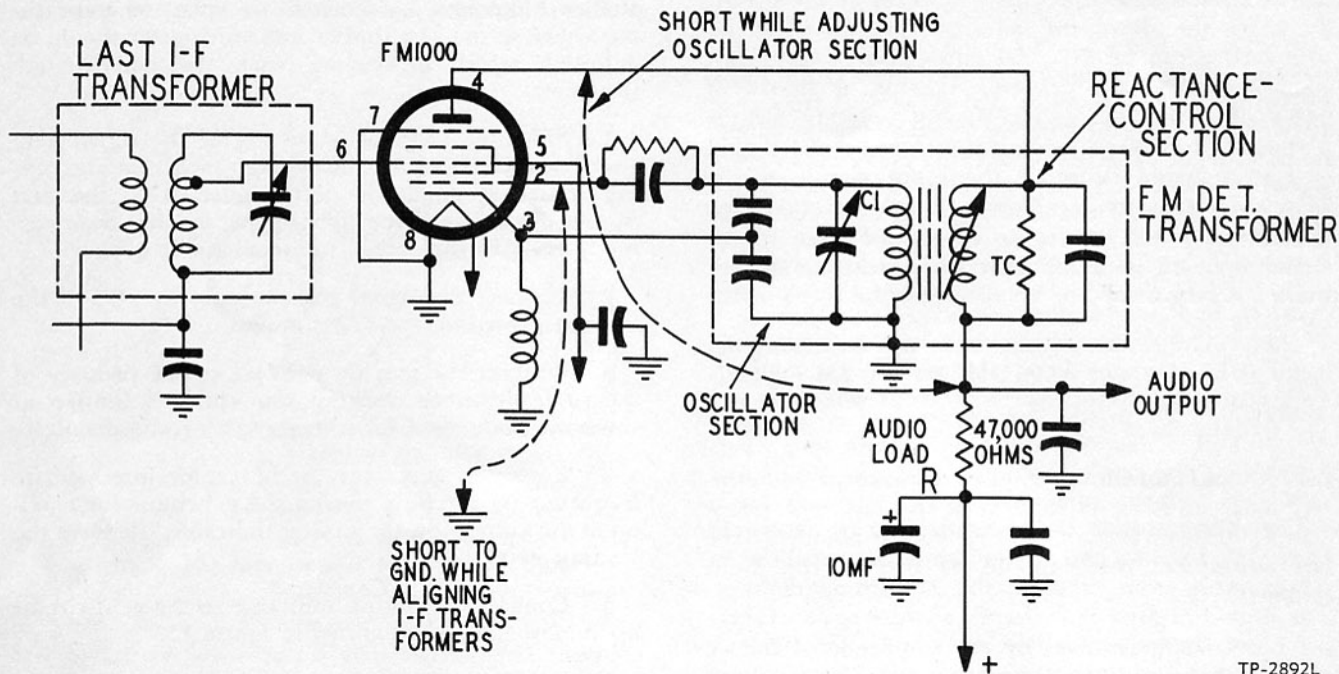
Figure 14. Advanced FM Detector Circuit
