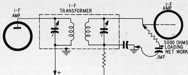
Figure 9. I-F Transformer with Loading Network Connected
